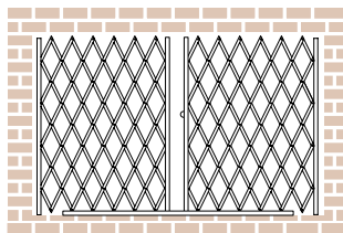
Pair Gate: Fixed bottom track. Max. Width: 16' Max. Height: 12' | Min. height: 31"
