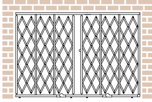
Pair Gate: Fixed top track and fold away bottom track. Max Width: 32' | Max. Height: 12'
