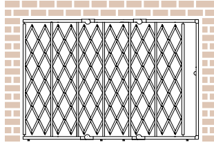
Single Gate: Fold away top track and fold away bottom track. Max Width: 16' | Max. Height: 7'6"
