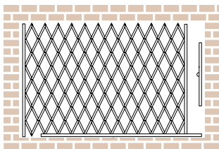
Single Gate: Fixed bottom track. Max. Width: 8' Max. Height: 12' | Min. height: 31"
