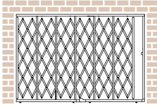
Single Gate: Fixed top track and fold away bottom track. Max Width: 16' | Max. Height: 12'
